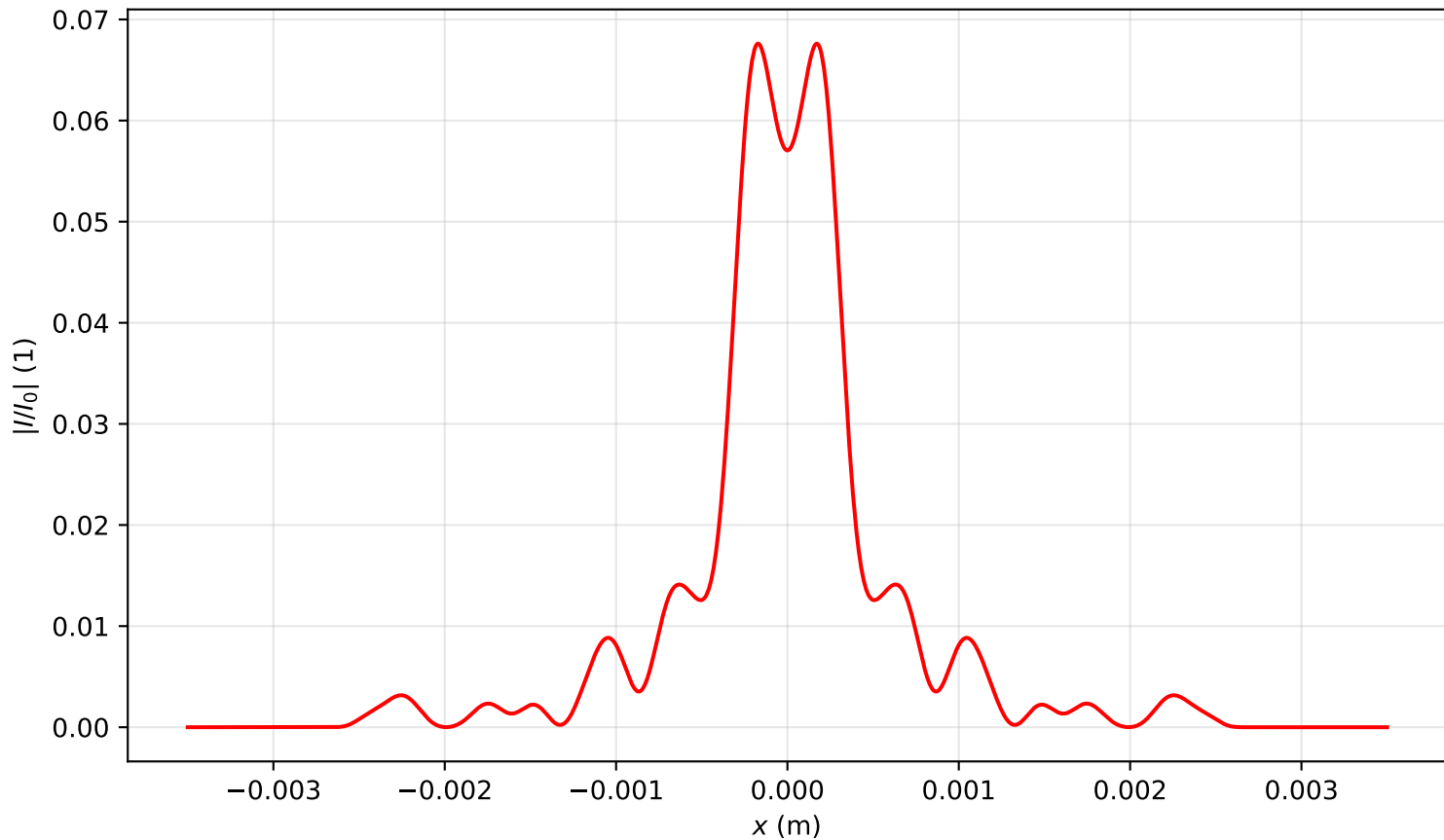
Intensity profile I(x, y = 0, z = 3.503)/I_0 , P_{in}=8.0P_{cr} , artificial time
